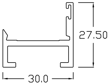
YC-2A Perimeter Frame
