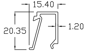
SLIM COVER
