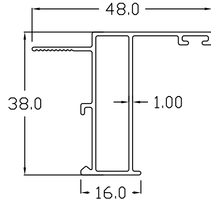
38 - 2 ( PANEL )
