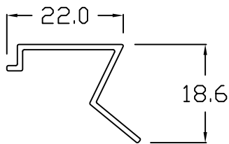
YC-12 Moulding
