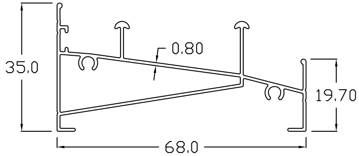
DOUBLE SILL
