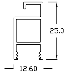
ASW - 21 SCREEN FRAME
