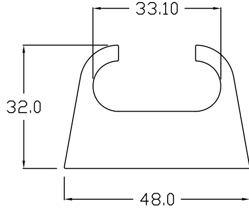
ED - 101BB PUSH BAR BRACKET
