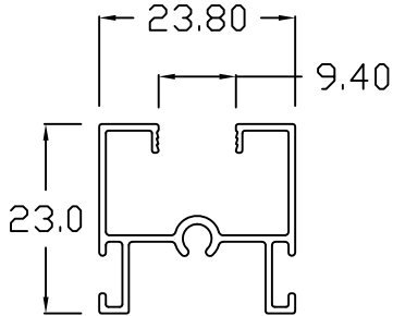
SD - 133 TOP RAIL
