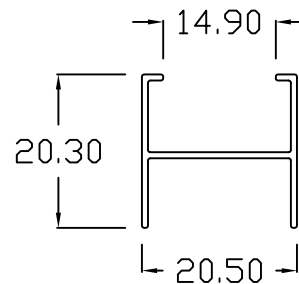
RPC 12149 SCREEN ASTRAGAL
