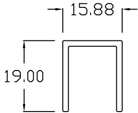
UC - 3/4 x 5/8
