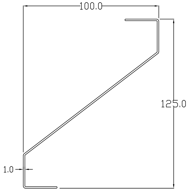
BIG LOUVER 125MM
