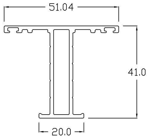
CLEO 47 YC Heavy Duty center panel
