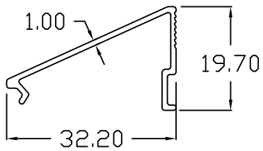
YC - 50 -12 S6 SMALL SLANT
