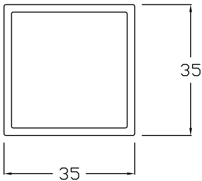
SQ. TUBE - 1 3/8 x 1 3/8
