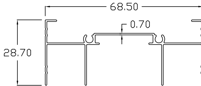
DOUBLE HEAD
