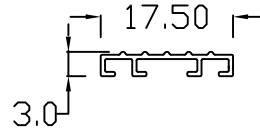
SF - 750D SCREEN FRAME 3/4 D/C
