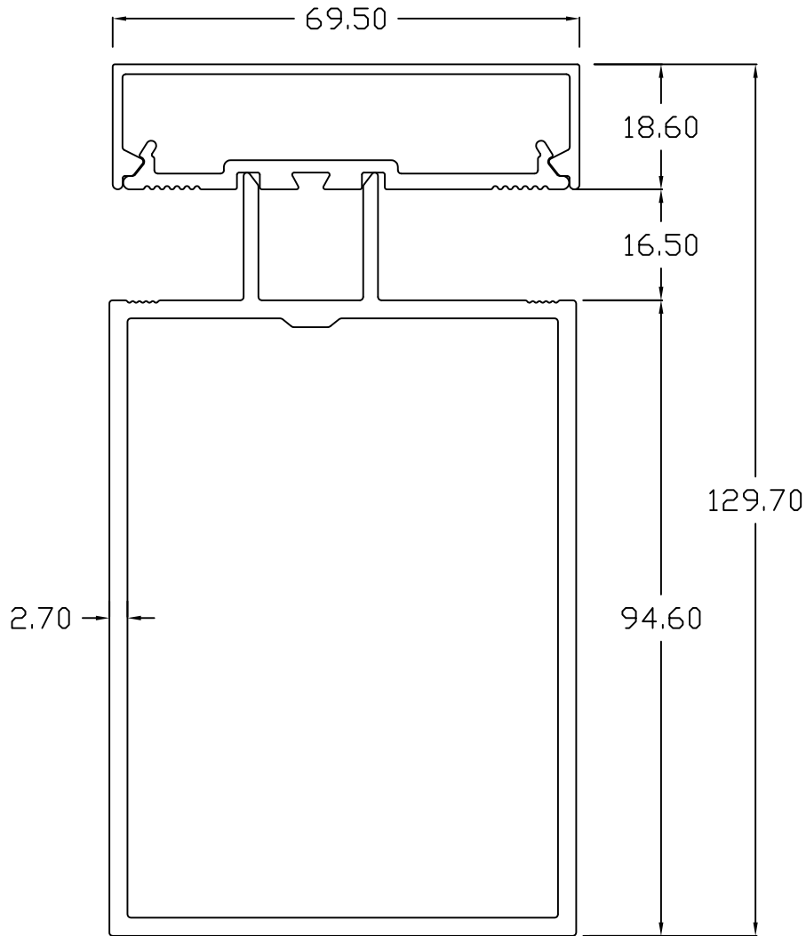
BIG MULLION
