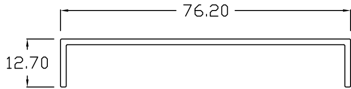
CT - 1/2 x 3
