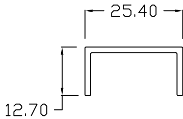
CT - 1/2 x 1
