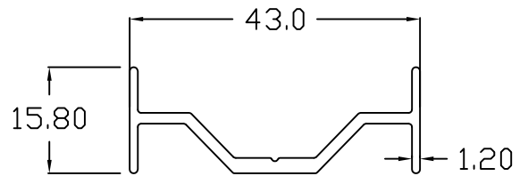
SLOT BRACKET
