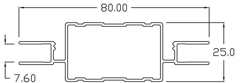
SF - 302 AMPLIMESH DOUBLE
