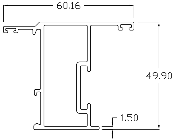
LYC - 2B PANEL FRAME ( MULTI - POINT LOCK )
