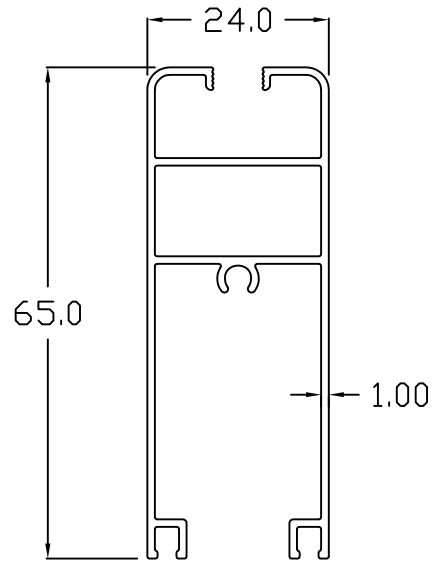
90005 BOTTOM RAIL
