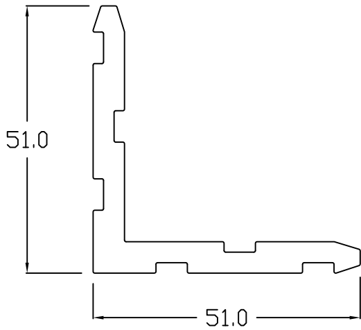
PC - 11288 Cornerstake 2 X 2
