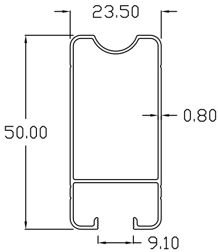
LOCKSTILE
