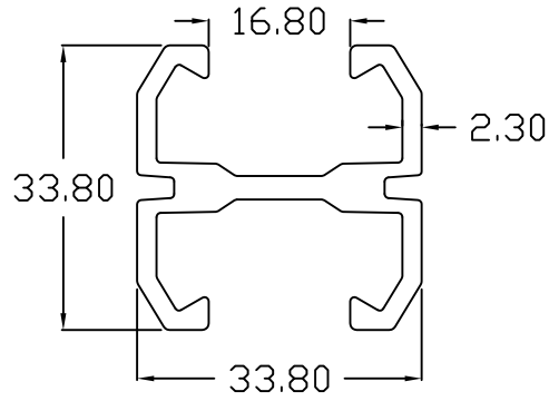
DOUBLE C
