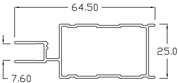
SF - 301 AMPLIMESH SINGLE
