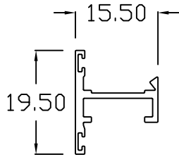
YC-1 Transom Bar
