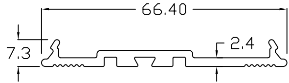
AMAC -A100 ADAPTER Mullion
