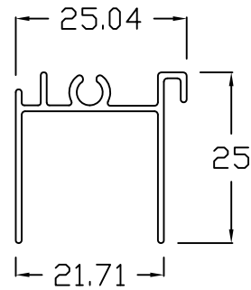
SD - 137 SCREEN HEAD
