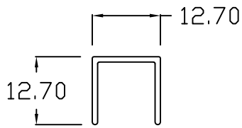
CT - 1/2 x 1/2
