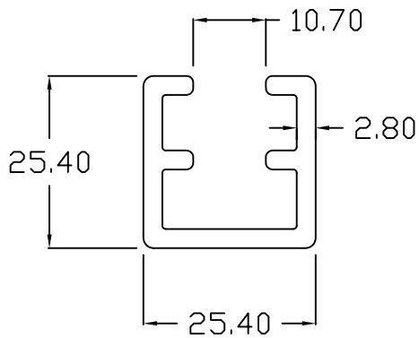
SOLAR / SIGNAGE SECTION
