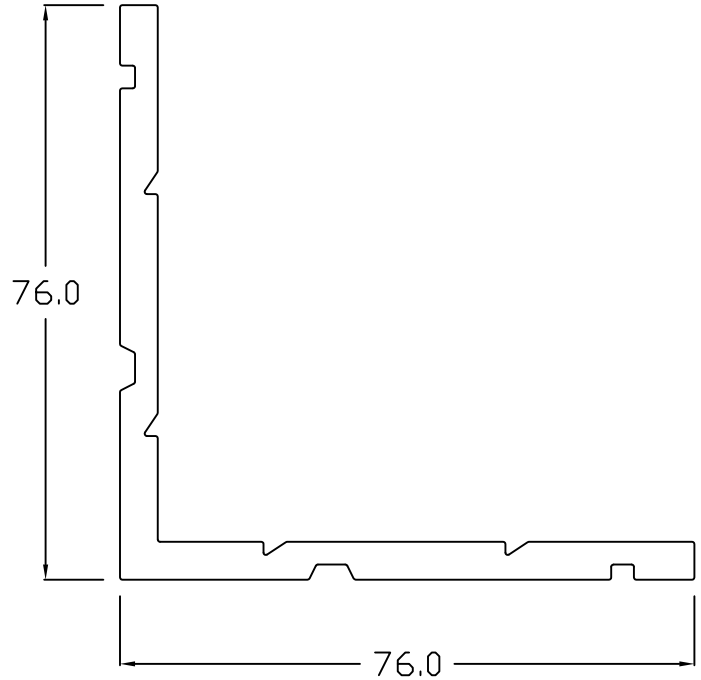
YC-17 Cornerstake 3 X 3
