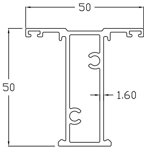
LYC - 4 CENTER MULLION
