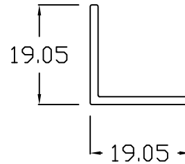
ANGLE - 3/4 x 3/4
