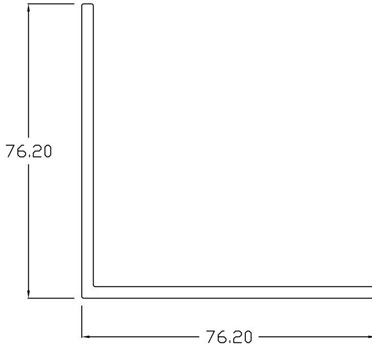
ANGLE - 3 x 3
