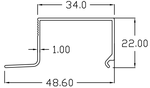
50-12 BIG SQUARE
