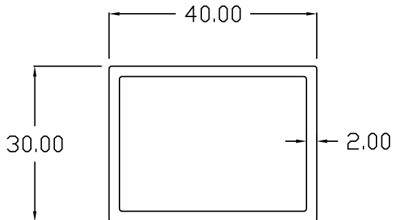
RECT. TUBE - 30mm x 40mm
