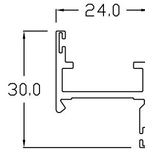
YC-2 Vent Frame Panel
