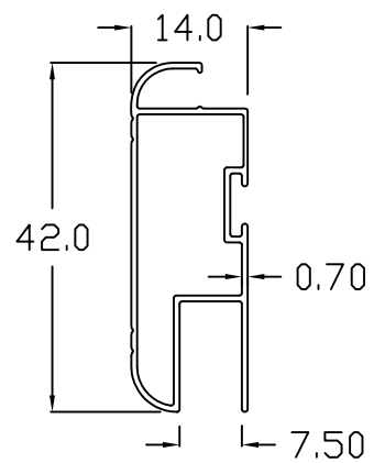
SCREEN FRAME
