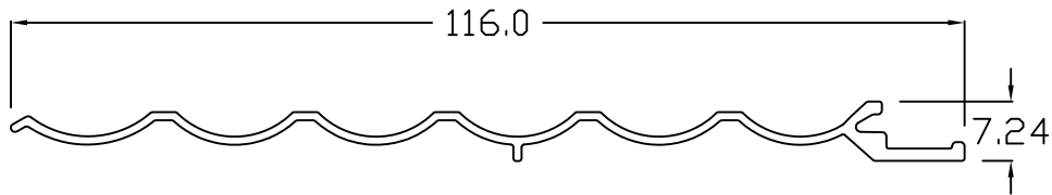
YP 100 BUS BODY SKIN
