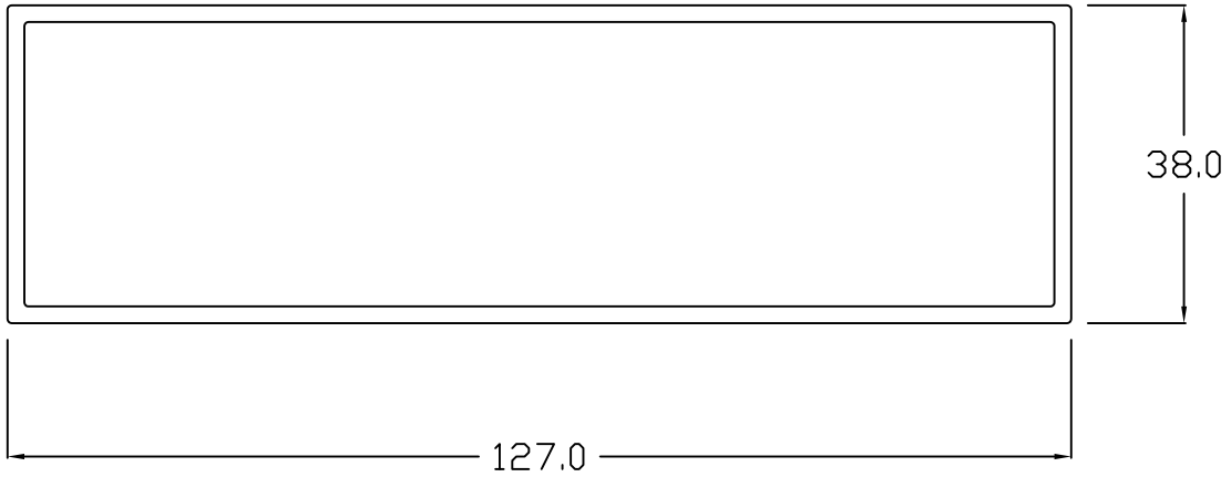
RECT. TUBE - 1 1/2 x 5
