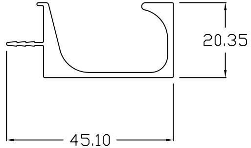
Drawer Handle Big
