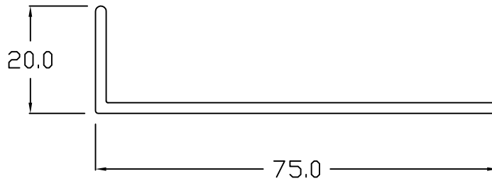
ANGLE - 20mm x 75mm
