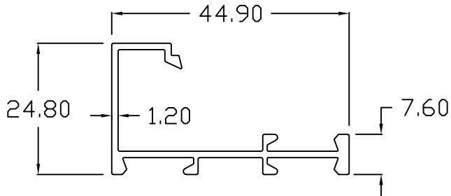
SLIM BASE
