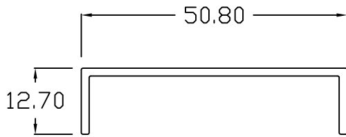
CT - 1/2 x 2
