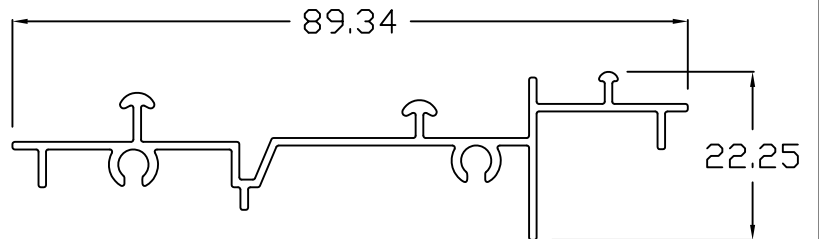
SD - 145 DOUBLE SILL W/ SCREEN
