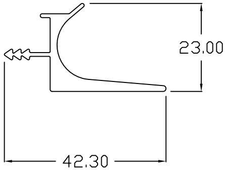
Drawer Handle Small
