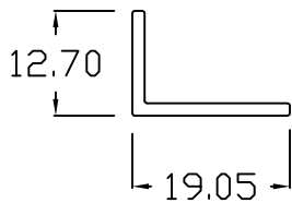
ANGLE - 1/2 x 3/4
