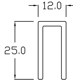
UC - 25 mm x 12 mm
