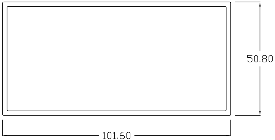
RECT. TUBE - 2 x 4
