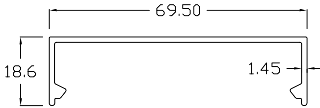
AMAC -C100 COVER Mullion
