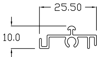
SD - 138 SCREEN SILL
