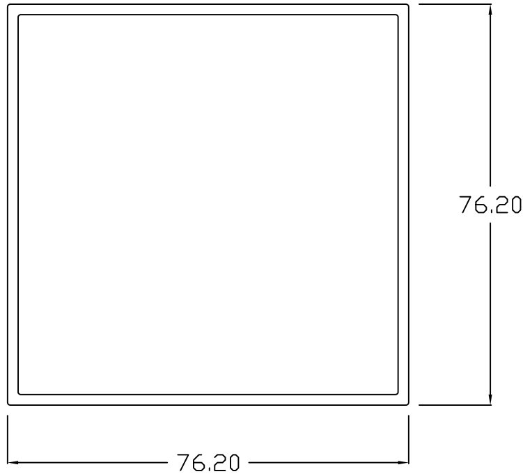
SQ. TUBE - 3 x 3
