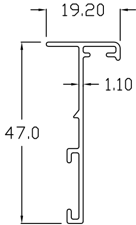
FRAME
