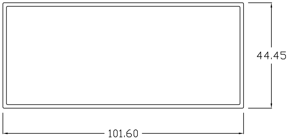
RECT. TUBE - 1 3/4 x 4
