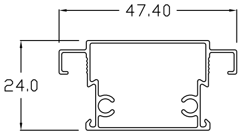
SF - 106 B CROSSBAR W/ SCREWHOLE
