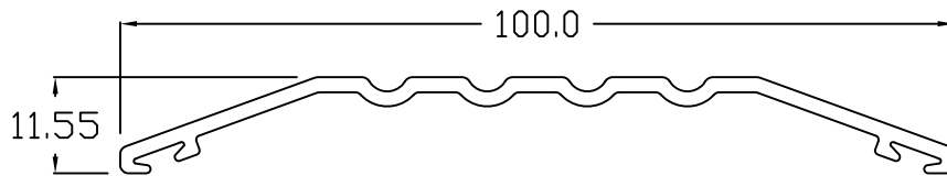
ED - 104 THRESHOLD 4"
