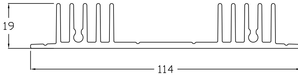
SINGLE HEATSINK
