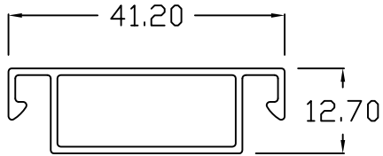
SF - 105 SCREEN CROSSBAR
