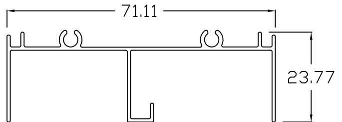
SD - 132 DOUBLE HEAD
