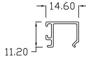
EF-114A SNAP ON COVER
