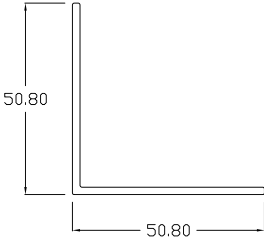
ANGLE - 2 x 2
