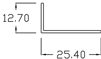
ANGLE - 1/2 x 1
