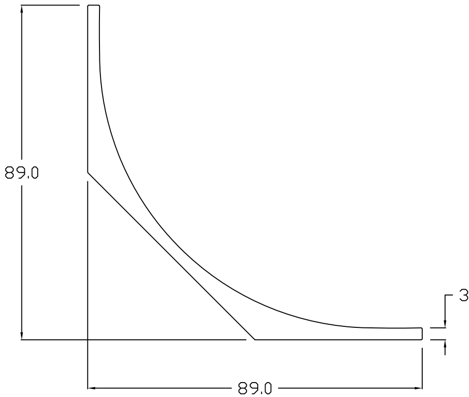
COVE RADIUS 2 "
