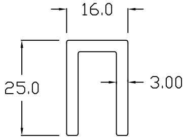
UC - 25 mm x 16 mm
