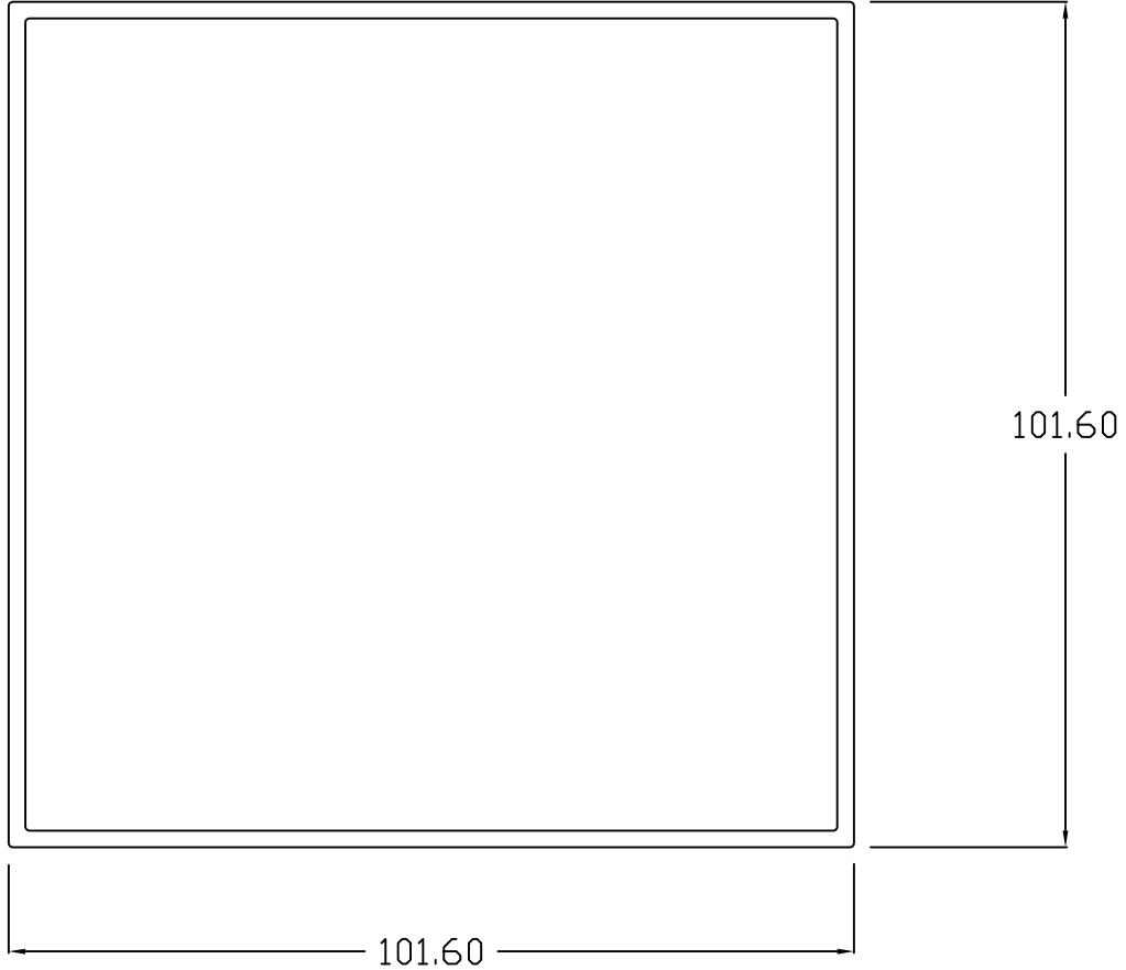
SQ. TUBE - 4 x 4
