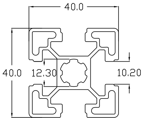
40 x 40
