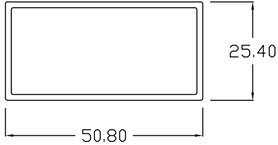
RECT. TUBE - 1 x 2
