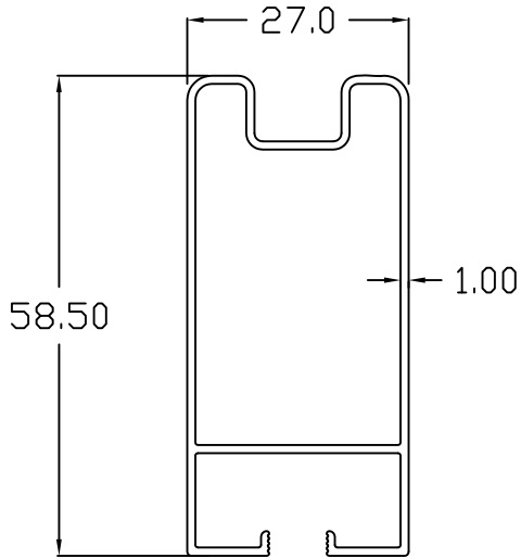
90006 LOCKSTILE
