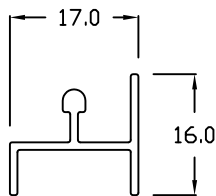
ASW - 22 SCREEN SILL
