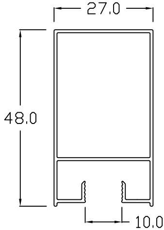
SD - 103 LOCKSTILE
