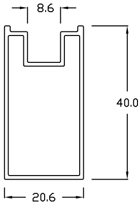
ASW - 6 LOCKSTILE
