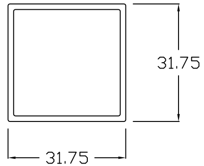
SQ. TUBE - 1 1/4 x 1 1/4
