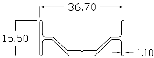
SLOT BRACKET
