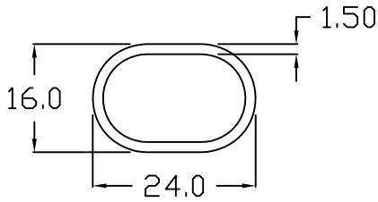
OVAL TUBE - 16mm x 24mm
