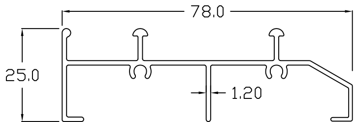
9008 DOUBLE FLAT SILL
