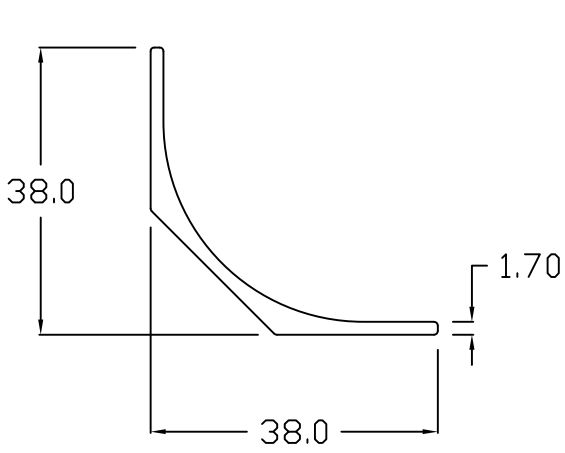
COVE RADIUS 1 1/2 "
