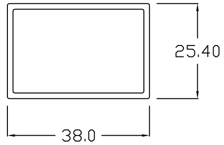
RECT. TUBE - 1 x 1 1/2
