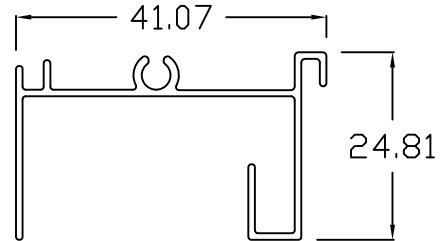
SD - 141 SINGLE HEAD
