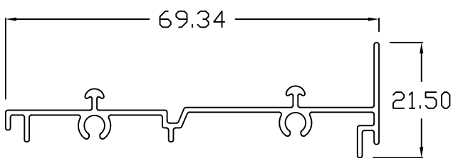
SD - 131 DOUBLE SILL
