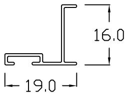
JW - 6105 BUMPER
