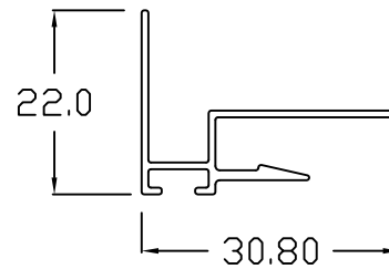
SD - 107 POCKET INTERLOCKER
