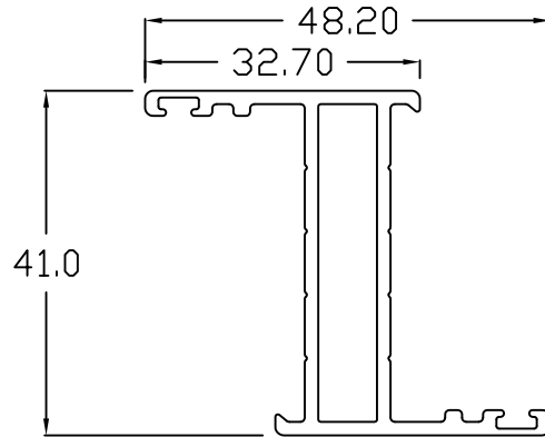
CLEO 46 YC Heavy Duty vent frame
