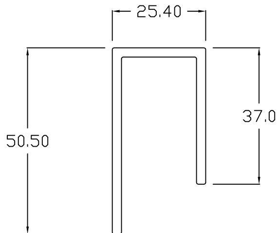
UC - 50 mm x 25 mm x 37 mm
