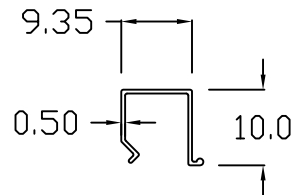
SF - 102 CLIP
