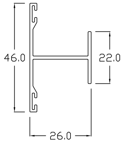
YC-4 Center Frame
