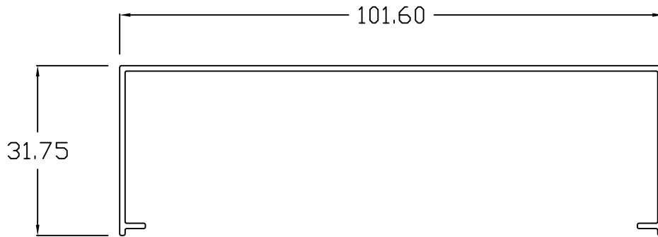
EF - 111C SPLIT TUBE
