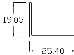
ANGLE - 3/4 x 1
