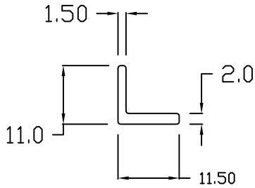
ANGLE - 11mm x 11.5mm
