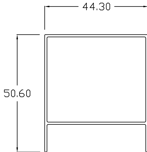
ED - 102 TOP RAIL
