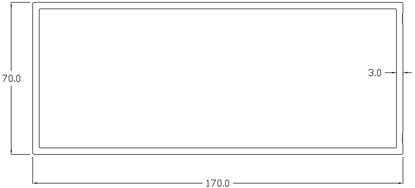
RECT. TUBE - 70mm x 170mm
