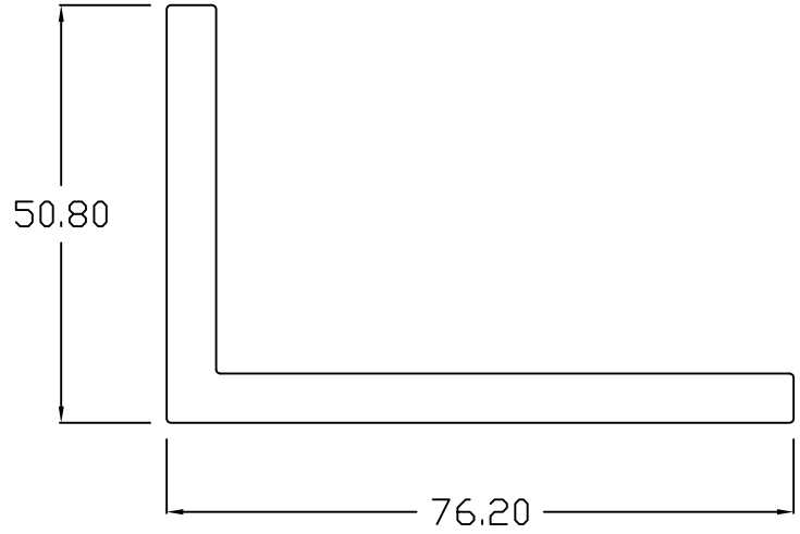
ANGLE - 2 x 3
