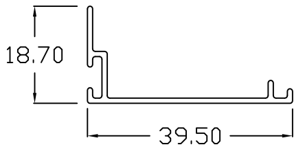
SD - 144 STEP SILL
