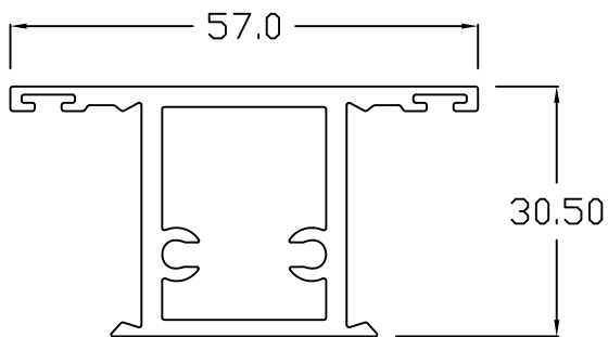
YC-18 Center Mullion
