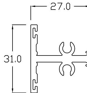
YC-16 Muntin
