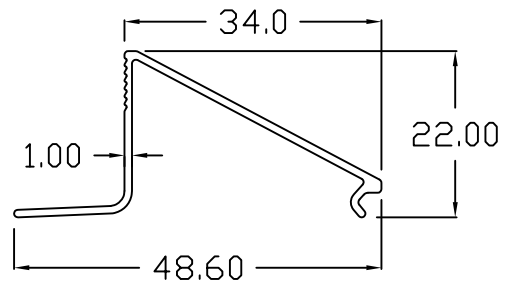
BIG SLANT
