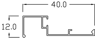
EF-114 SNAP ON BASE
