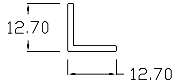
ANGLE - 1/2 x 1/2
