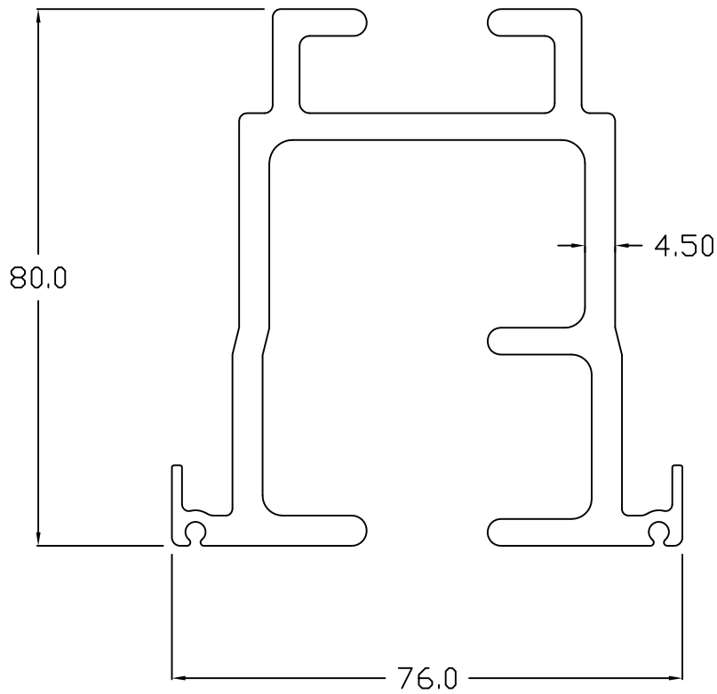
RAIL TRACK
