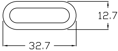
ED - 101PB PUSH BAR W/ HOLE
