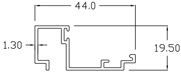
SNAP ON BASE 1/2
