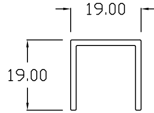
UC - 3/4 x 3/4
