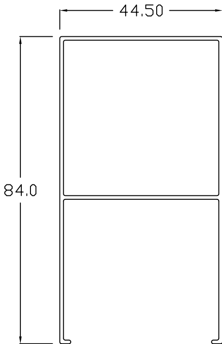
ED - 101 BOTTOM RAIL
